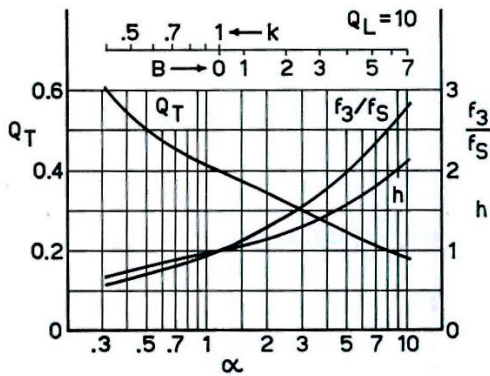
Fig. 10. Alignment chart for vented-box systems with Q_B = Q_L = 10 .
