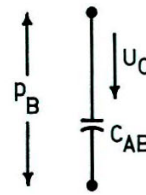
Fig. 2. Acoustical analogous circuit of lossless enclosure.
