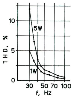
Fig. 8. Measured total harmonic distortion of vented-box system.
