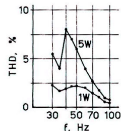
Fig. 6. Measured total harmonic distortion of closed-box system.
