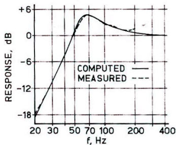
Fig. 5. Frequency response of closed-box system.
