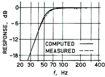
Fig. 7. Frequency response of vented-box system.
