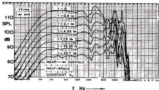
Fig. 9. Experimental measurements performed to check Eq. (7) and Fig. 4. The source is a 4.5-in (11.4-cm) wide-range driver, mounted in a 395-in 3 (6473-cm 3 ) closed box, flush mounted in the center of a 4- by 8-ft (1.2- by 2.4-m) sheet of ¾-in (1.9-cm) plywood. Seven anechoic axial frequency response measurements were made with the measurement microphone the indicated distance from the diaphragm. The distances chosen correspond to low-frequency axial attenuations of 0, -5, -10, -15, -20, -25, and -30 dB relative to the nearfield pressure at r = 0 .
