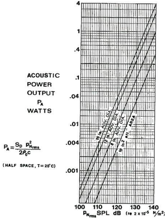
Fig. 6. Total radiated sound power P_A of a rigid circular piston radiating into a half-space to nearfield sound pressure level measured at points close to center of piston, for low frequencies such that ka < 1 . The following piston sizes are plotted: 10-in 2 (64.5-cm 2 ) effective (actual) area, 8-in (20.3-cm) advertised diameter (6.2-in (15.7-cm) effective diameter), 12-in (30.5-cm) advertised diameter (9.8-in (26.9-cm) effective diameter), and 15-in (38-cm) advertised diameter (12.6-in (32-cm) effective diameter).
