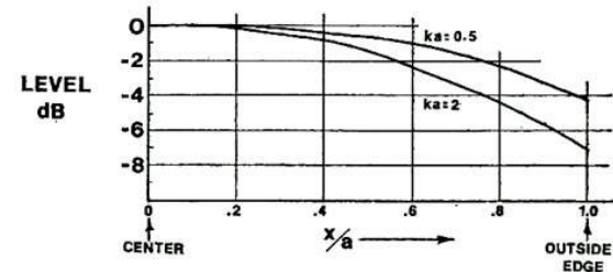
Fig. 5. Normalized nearfield sound pressure distribution on surface of a rigid circular piston vibrating in an infinite flat baffle, for ka = 0.5 and 2. The distribution exhibits circular symmetry and is only a function of the radial distance from the center to the edge of the piston (after [4]).
