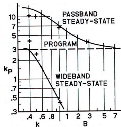
Fig. 18. Power rating constant k_P for vented-box loud-speaker system as a function of response shape. Solid lines are for lossless systems; crosses represent systems with Q_L = 5 .
