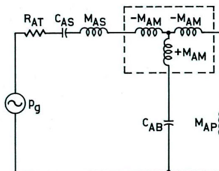
Fig. 22. Acoustical analogous circuit of lossless vented-box loudspeaker system modified to include effects of diaphragm-vent mutual coupling.
