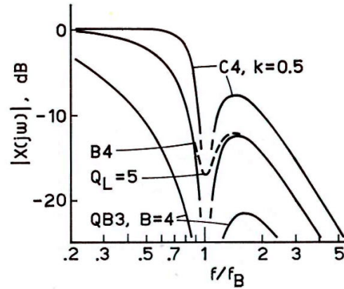
Fig. 17. Normalized diaphragm displacement of vented-box system driver as a function of normalized frequency for several typical alignments (from simulator).
