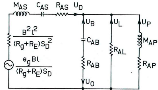
Fig. 1. Acoustical analogous circuit of vented-box loudspeaker system.
