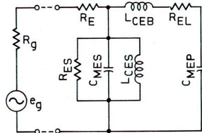
Fig. 3. Simplified electrical equivalent circuit of vented-box loudspeaker system.
