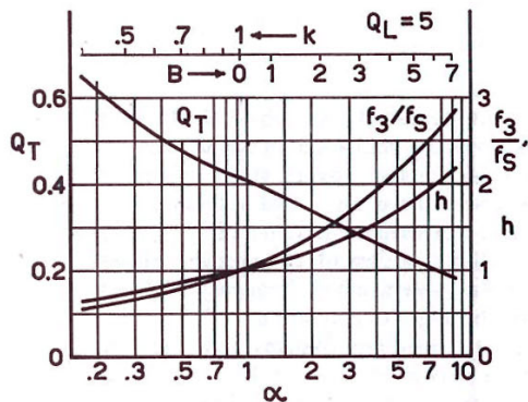
Fig. 12. Alignment chart for vented-box systems with Q_B = Q_L = 5 .
