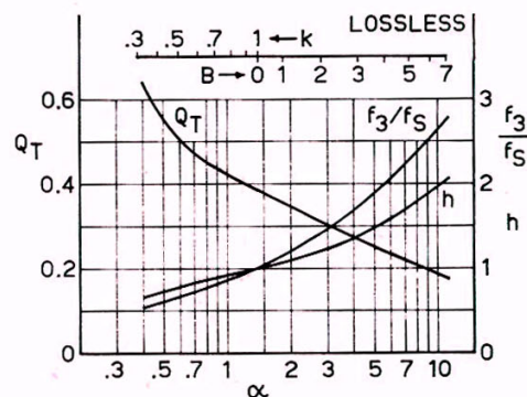
Fig. 6. Alignment chart for lossless vented-box systems.
