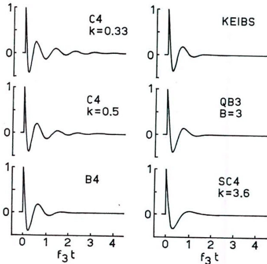
Fig. 14. Normalized step response of vented-box loudspeaker system (from simulator).
