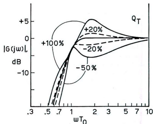
Fig. 7. Variations in frequency response of lossless B4-aligned vented-box system for misalignment of Q_T (from simulator).
