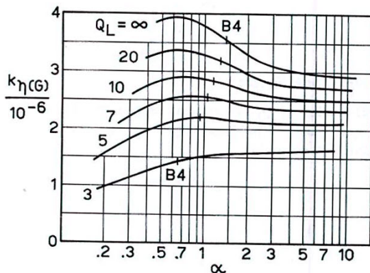
Fig. 15. Response factor k_{\eta(G)} of efficiency constant for vented-box loudspeaker system as a function of a (system compliance ratio) for several values of enclosure Q_L .
