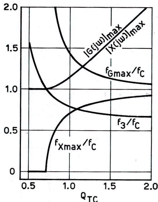
Fig. 5. Normalized cutoff frequency, and normalized frequency and magnitude of response and displacement peaks, as a function of total Q for the closed-box loudspeaker system.
