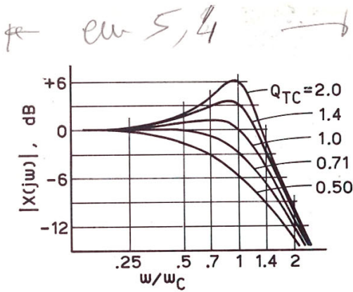
Fig. 9. Normalized diaphragm displacement of closed-box system driver as a function of normalized frequency for several values of total system Q .
